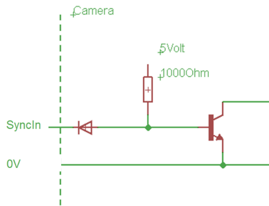
Figure 10: Sync In Input Schematics
