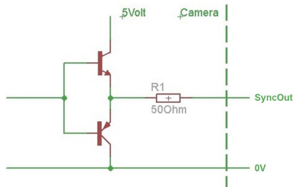
Figure 11: Sync Out Output Schematics
